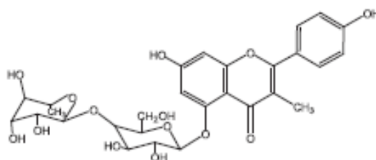
4',5,7-Trihydroxy-3-C-methylflavone-5-O-α-L-rhamnopyranosyl- (1→4)-O-β-D-galactopyranoside
