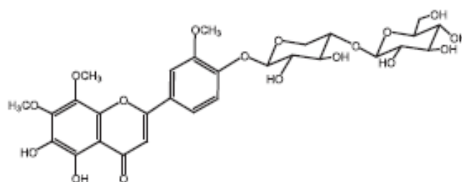
5,6-Dihydroxy-3',7,8-trimethoxyflavone-4'-O-β-D-glucopyranosyl- (1→4)-O-β-D-xylopyranoside
