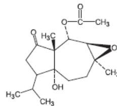
1α-Acetoxy-2β,3β-epoxy-6α-hydroxy-9-oxocarot-2-ene
