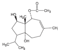
1α-Acetoxy-6α,9β-dihydroxycarot-2-ene
