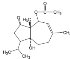
1α-Acetoxy-6α-hydroxy-9-oxocarot-2-ene
