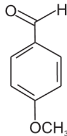
p -Anisaldehyde
