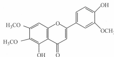
Anisomelin
