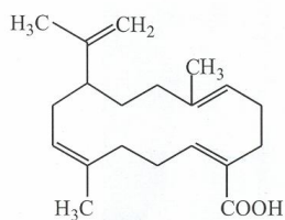
Malabaric acid
