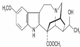
Voacristine and its isomer Isovoacristine
