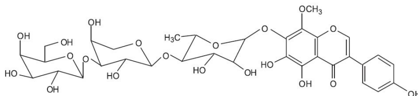
4',5,6,7-Tetrahydroxy-8-methoxyisoflavone-7- O - \beta -D-galactopyranosyl-(1 \rightarrow 3)- O - \beta -D-xylopyranosyl-(1 \rightarrow 4)- O - \alpha -L-rhamnopyranoside
